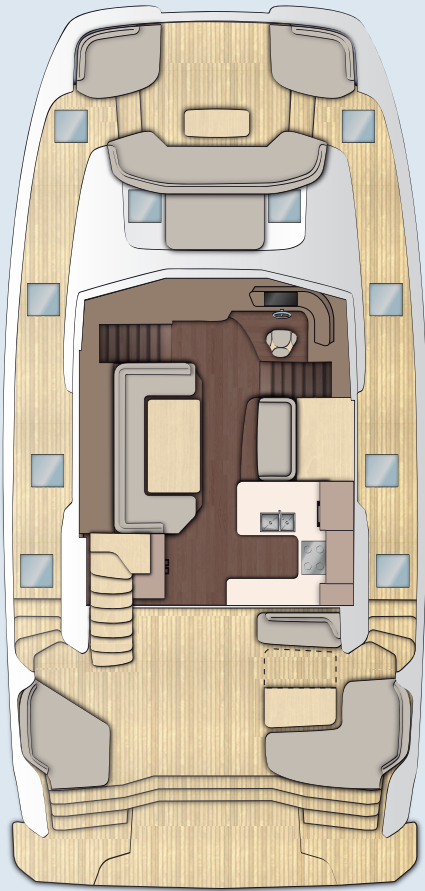
4 cabins version with standard aft lounge cockpit
