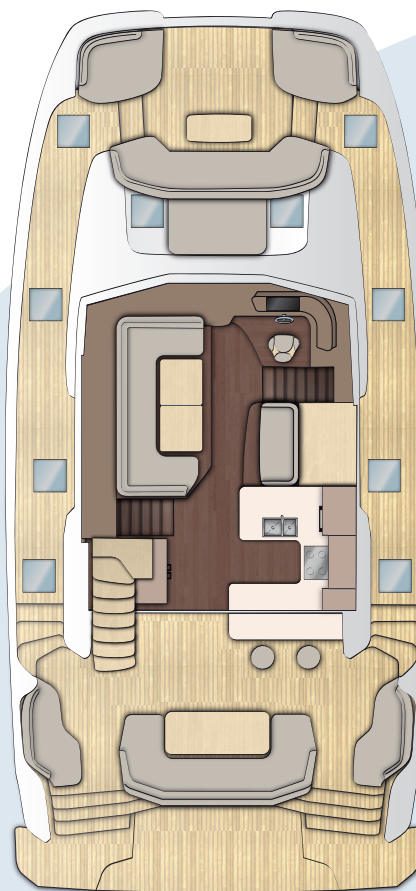
3 cabins version with optional aft deck layout
